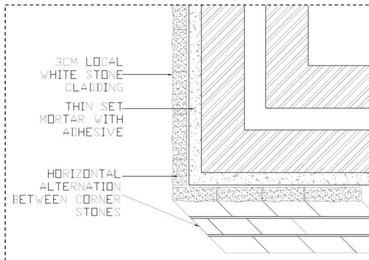
Typical Detail for cladding at corners
