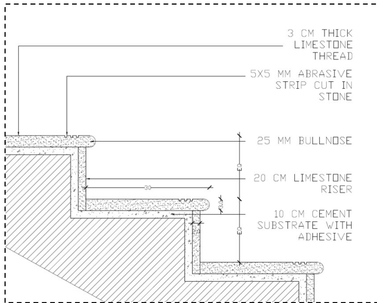
Typical Detail for stairs tiling
